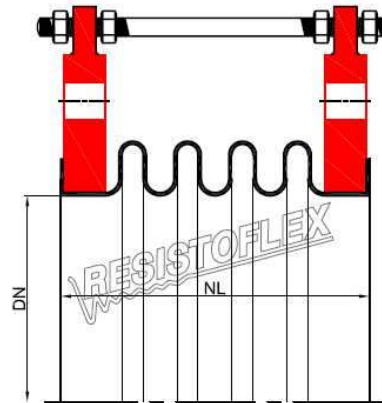
MEJ with Control Units for other lines
